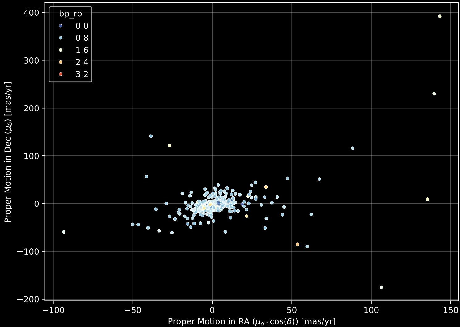
APOGEE DR17 Field: [K19_076+07] Proper Motion Diagram (n= 751)
