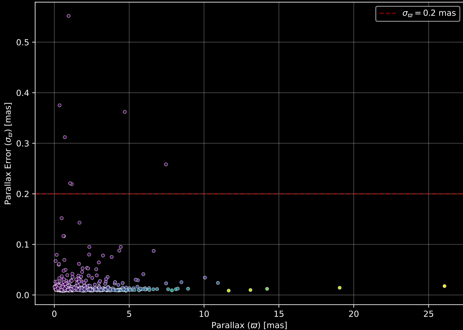
APOGEE DR17 Field: [K19_076+07] Parallax Quality (n= 751)
