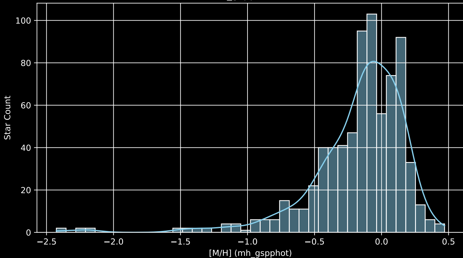
APOGEE DR17 Field: [K19_076+07] [M/H] (mh_gspphot) (n= 744)
