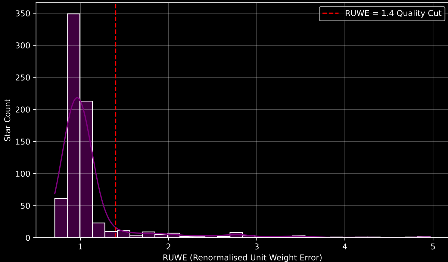
GAPOGEE DR17 Field [K19_076+07] RUWE Distribution (n= 728)
