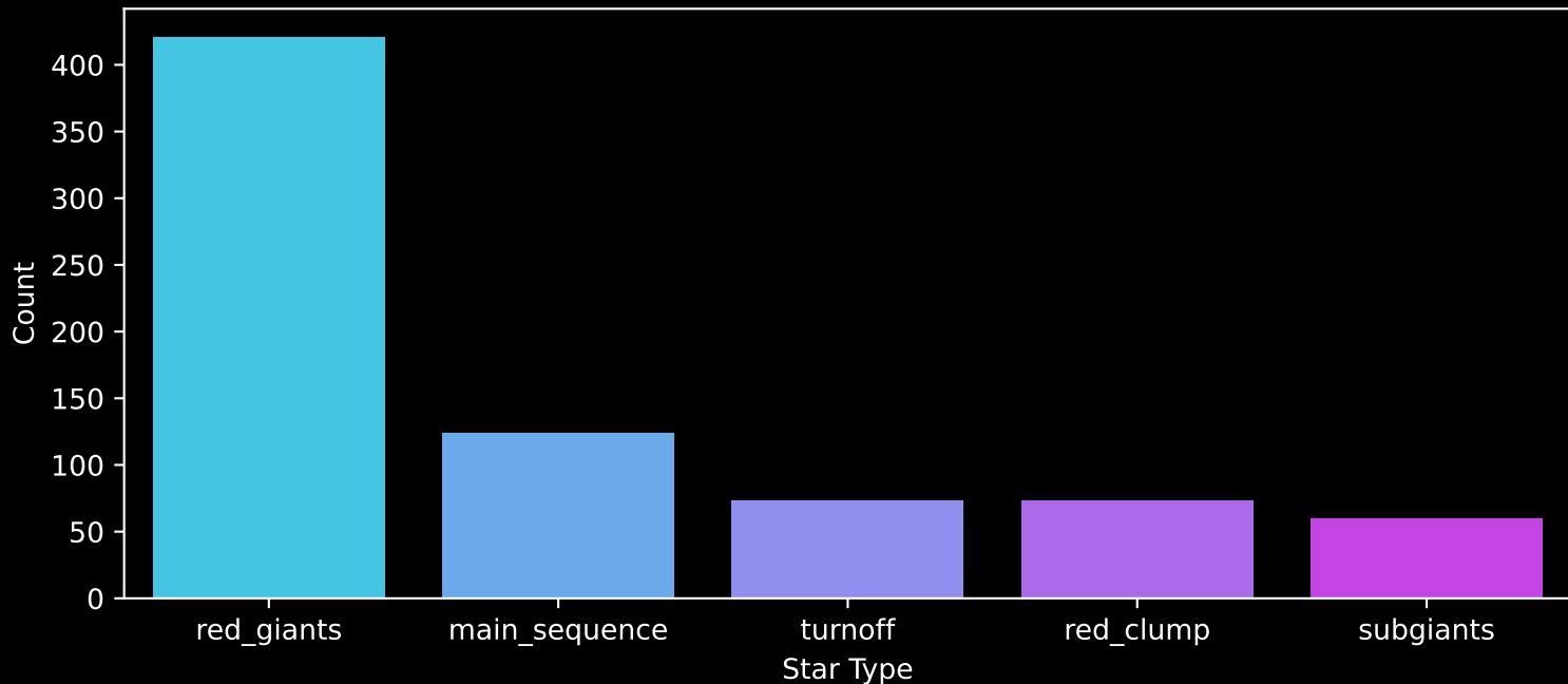
APOGEE DR17 Field: [K19_076+07] Count plot of Star Type
