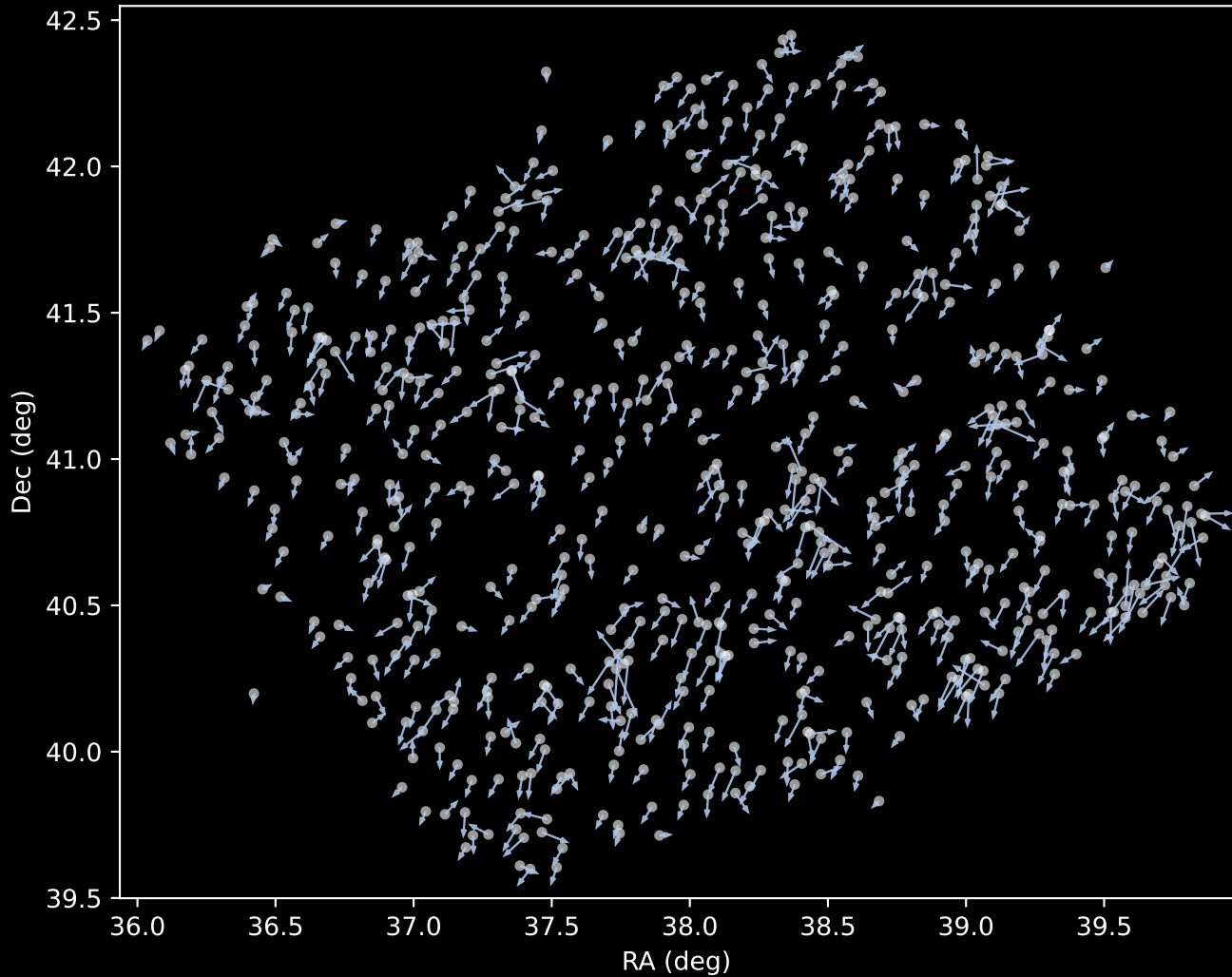
APOGEE DR17 Cluster 1 Proper Motion Vectors (n=646)
